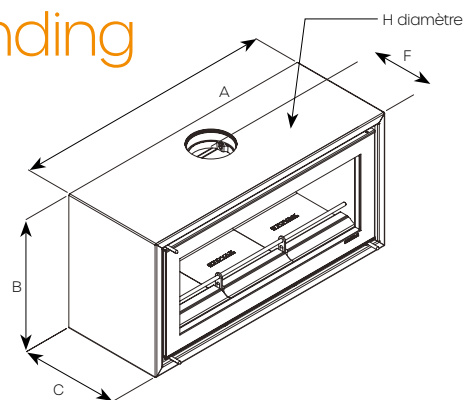
Dimensions Freestanding**
